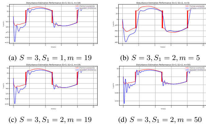
Fig. 20: Simulation1: Python-based disturbance estimation results with RBF compensation.
