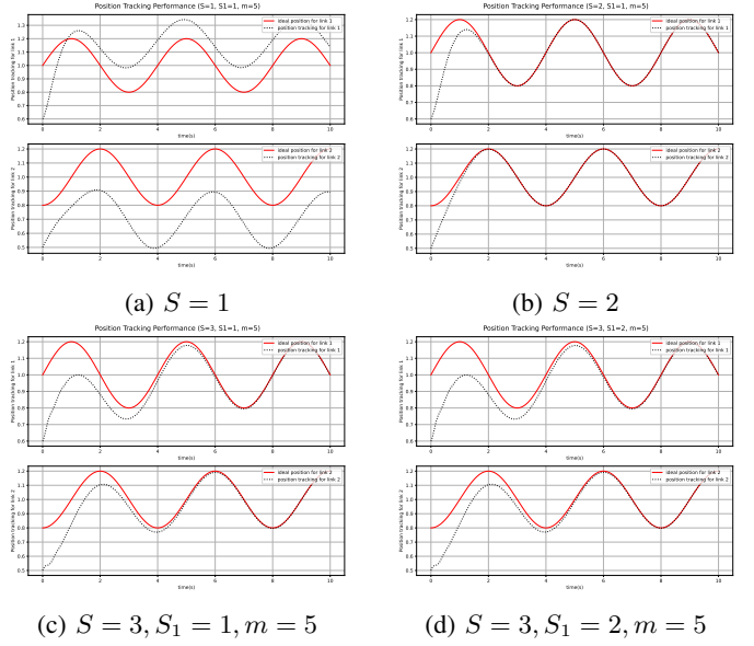
Fig. 21: Simulation2: Python-based position tracking results for the two-link manipulator.
