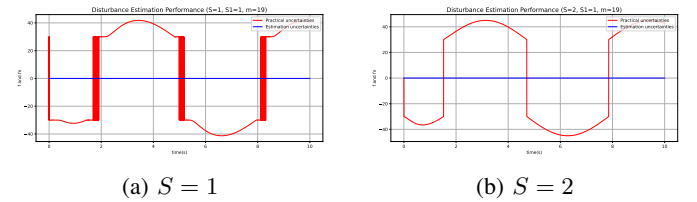
Fig. 18: Simulation1: Python-based disturbance responses for controllers without RBF compensation.
