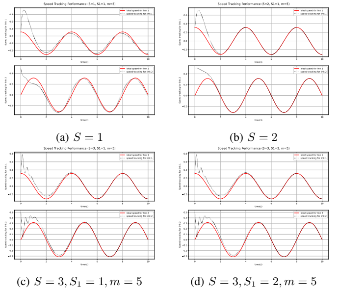
Fig. 22: Simulation2: Python-based velocity tracking results for the two-link manipulator.
