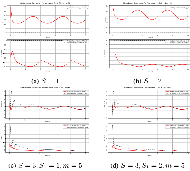
Fig. 24: Simulation2: Python-based disturbance estimation results for the two-link manipulator.
